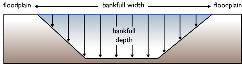
Figure 14. A stream channel cross section showing bankfull width and bankfull depth.
