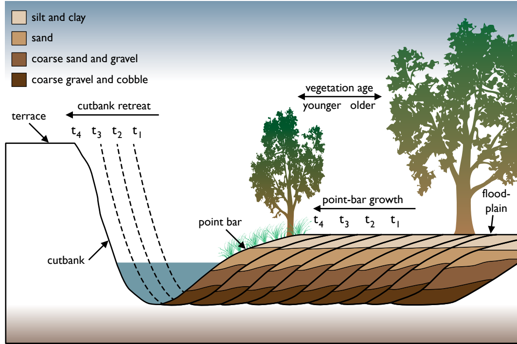
Figure 28. An idealized cross section through a point bar of a hypothetical meandering channel illustrates (1) gently sloping to convex upward form of the point-bar surface; (2) topographic continuity between the top of the point bar and the floodplain; (3) fining-upward sequence of sedimentary textures within the point bar; and (4) a constancy of channel cross-sectional area, indicating that the volume of erosion on the cutbank is approximately equal to the corresponding volume of sediment accumulated on the point bar over time (as suggested by channel position from time 1 ( t_1 ) through time 4 ( t_4 )).
